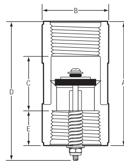
FIG. III Female Inlet x Female Outlet Option
