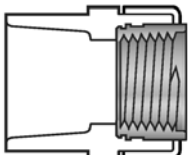
Transition Female Adapter Soc x Fipt With 316 Stainless Steel Thread Insert
